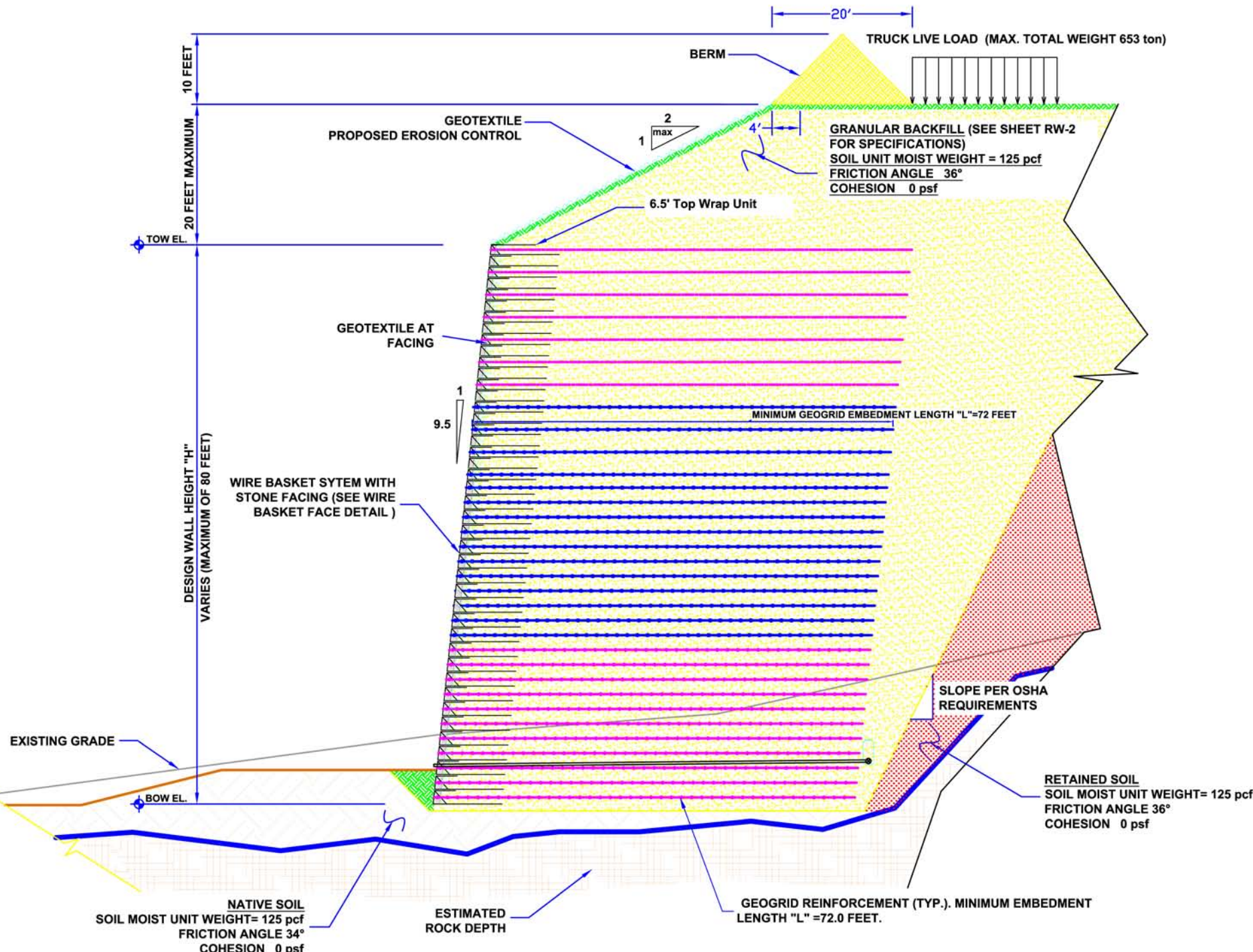
TYPICAL RETAINING WALL CROSS SECTION - "H" -80 FEET
